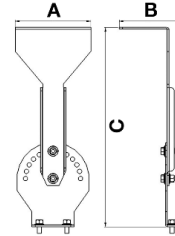
Wall-Mounted Hanger Set With 10° Angular Adjustment Steps Product Code : 3080656
