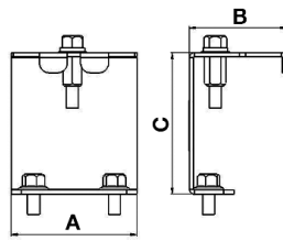
Revoled Poli Carbon Cable Tray and Wall Hanger Set Product Code : 3163476
