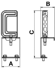
Revoled Poli Carbon Busbar Hanger Set Product Code : 3163889
